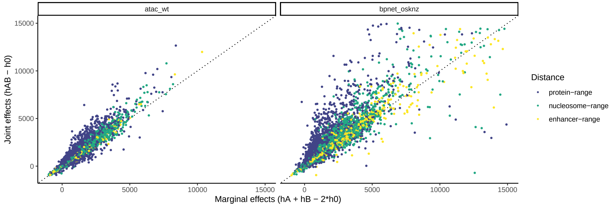
Sox2 vs Zic3
